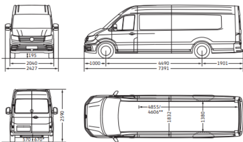
Crafter 35 ELWB High Roof
